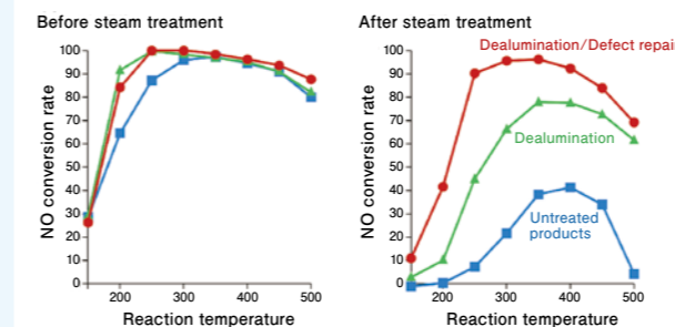
Results of catalyst testing
