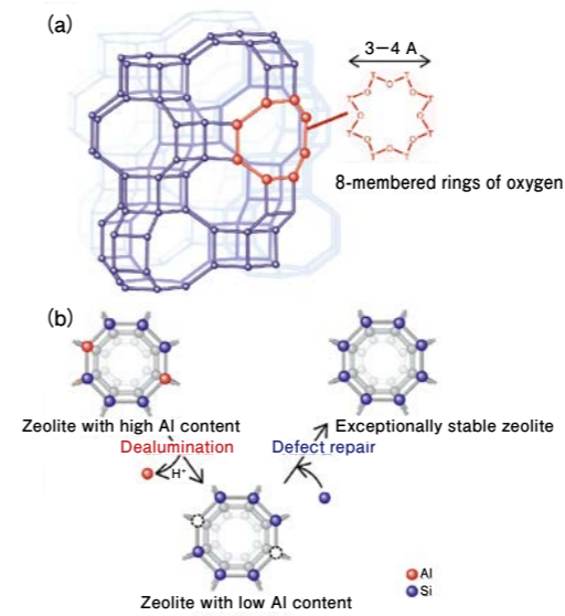
Schematic diagram of small pore zeolite composition tuning method
