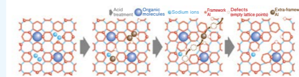
Mechanism of pore expansion and migration process
