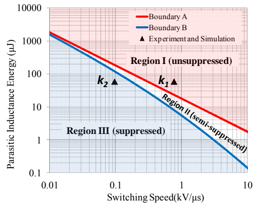
(d) Relationship between the parasitic inductance energy and switching speed
