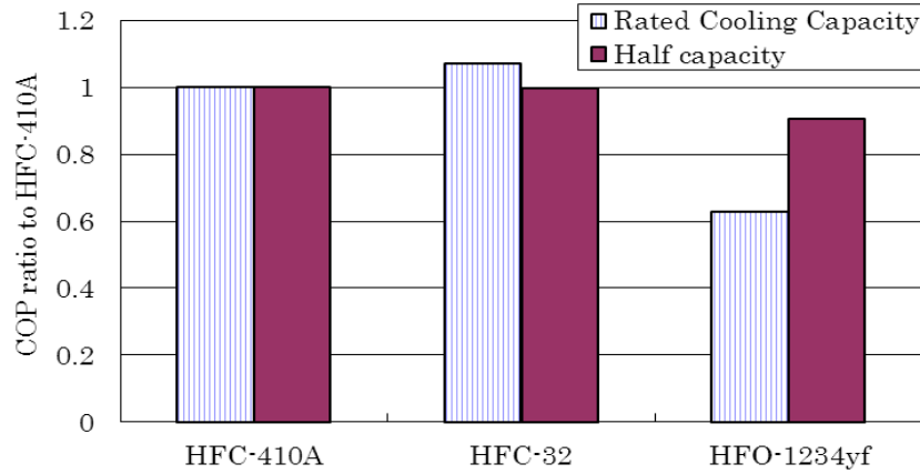
Fig. 4.1.8 COP ratio to HFC-410A at cooling mode
