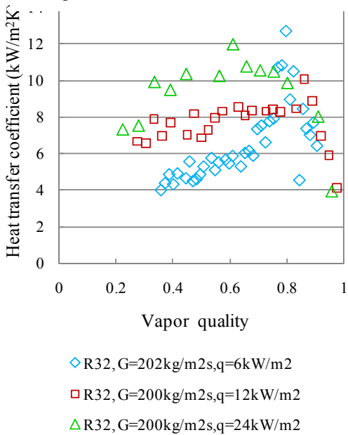
Fig. 1.3.2-7 Heat transfer coefficients at 200kg/m 2 s mass flux and 6 kW/m 2 heat flux
