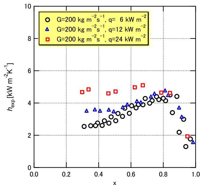
Figure 1.3.1.3. Effect of heat flux on local heat transfer coefficient
