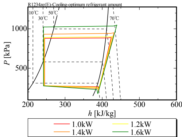
(e) HFO-1234ze(E)
