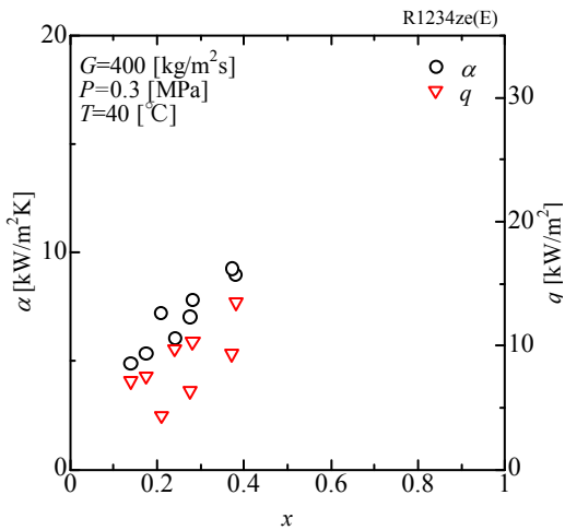
(a) HFO-1234ze(E)
