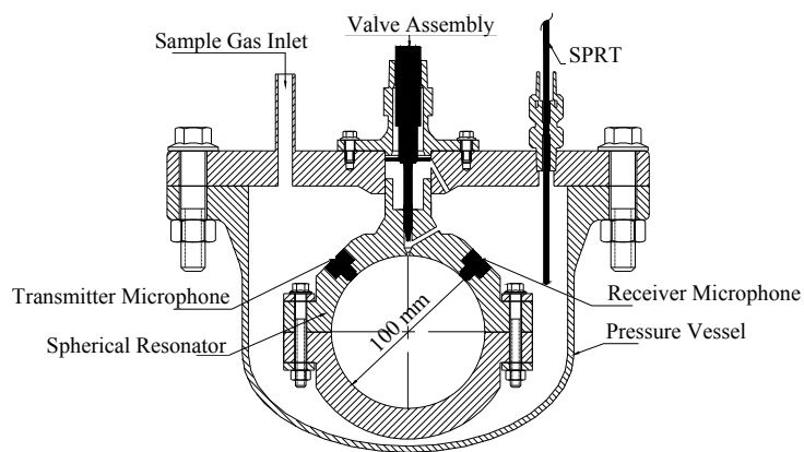
Fig.1.4.6 Cross-section view of the spherical acoustic resonator.
