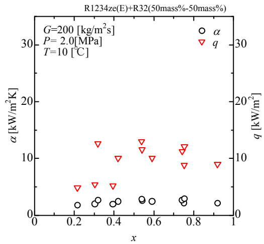
(b) HFO-1234ze(E)+R32(50mass%-50mass%)
